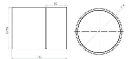
D10-L13-12w-18w-36w Surface Mounting IP54
