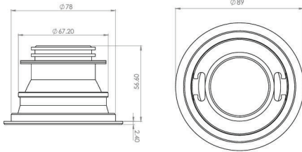
Narrow Brim D8-B1-6w Size 8 Bevel IP54
